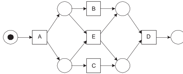
Fig. 2. A process model based on the event log shown in Table 1 discovered by the \alpha -algorithm [6].
