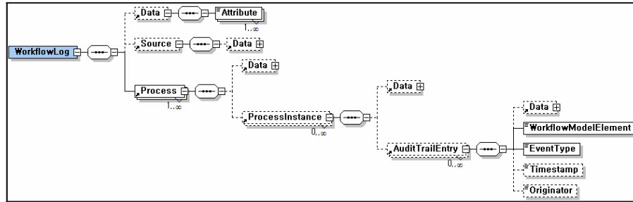
Fig. 4. MiSoN Workflow Mining Format (XML Schema).
