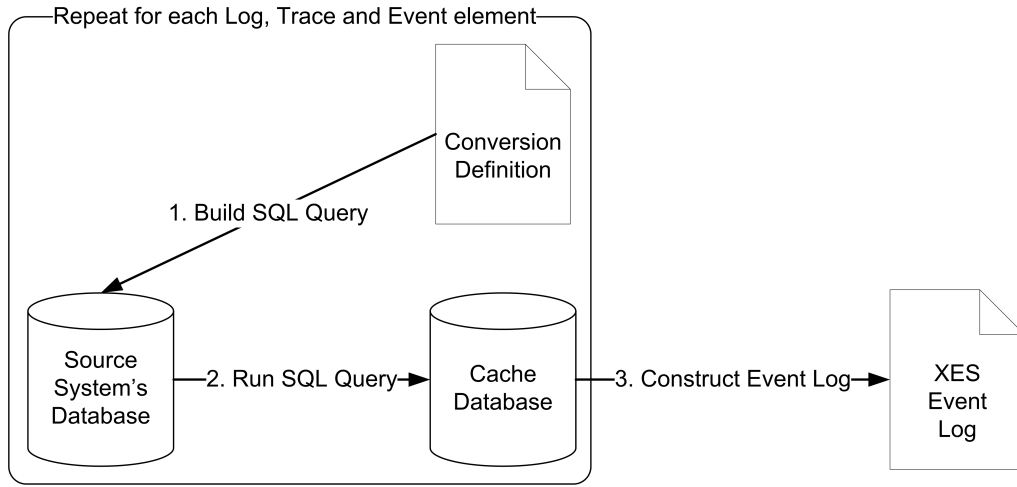
Figure 4.4: The three execution phases of the application.
