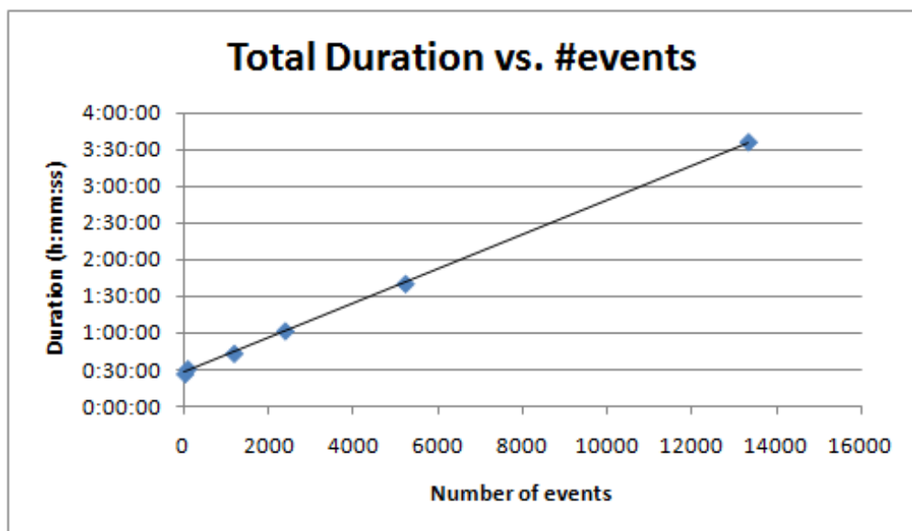
Figure 6.10: Case study 2: Conversion duration versus number of events.
