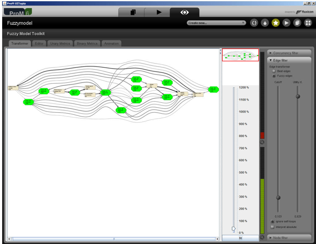
(b) Process model using the Fuzzy miner.
