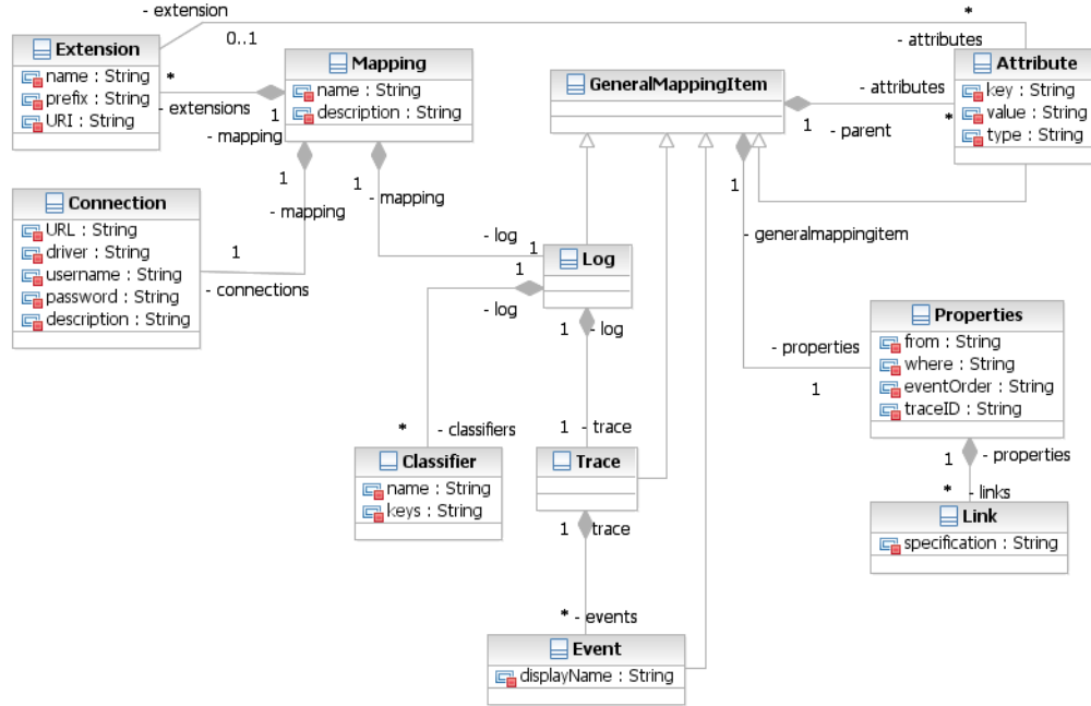
Figure 4.1: Class diagram of the domain model of the application.
