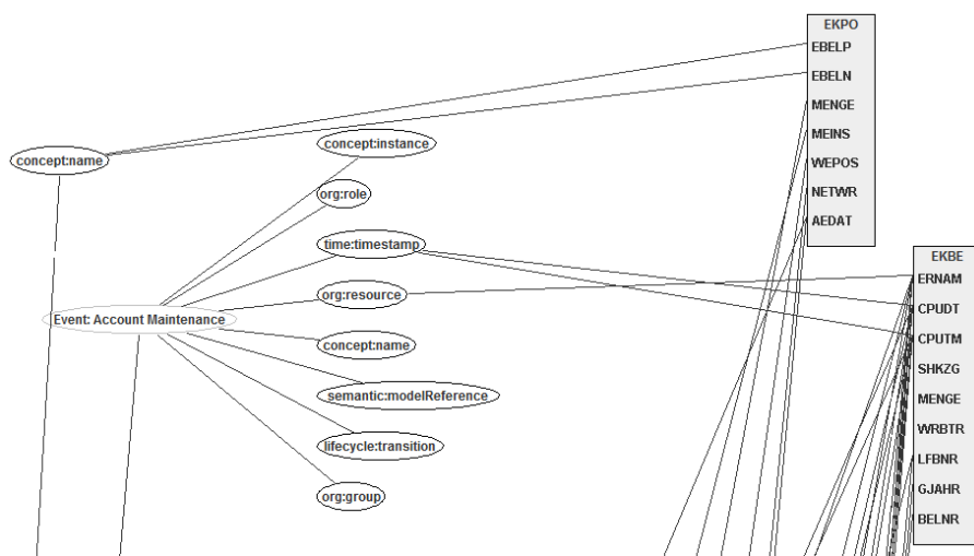
Figure 6.2: Part of the conversion visualization for case study 1.
