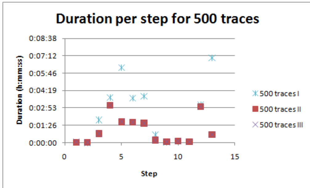
(a) Case study 1: Time per execution step for 500 traces.
