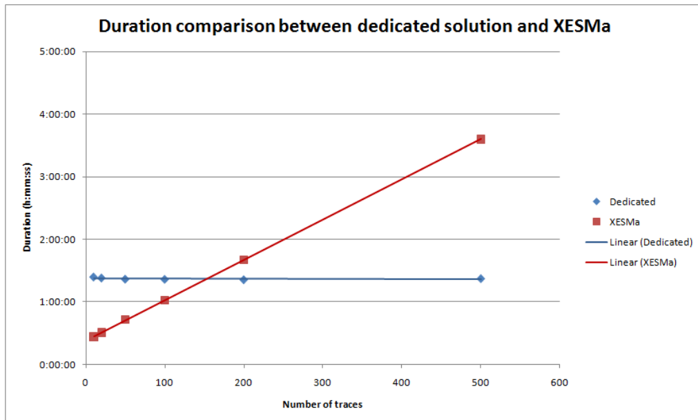
Figure 6.9: Case study 2: Comparison between the dedicated implementation and XESMa.
