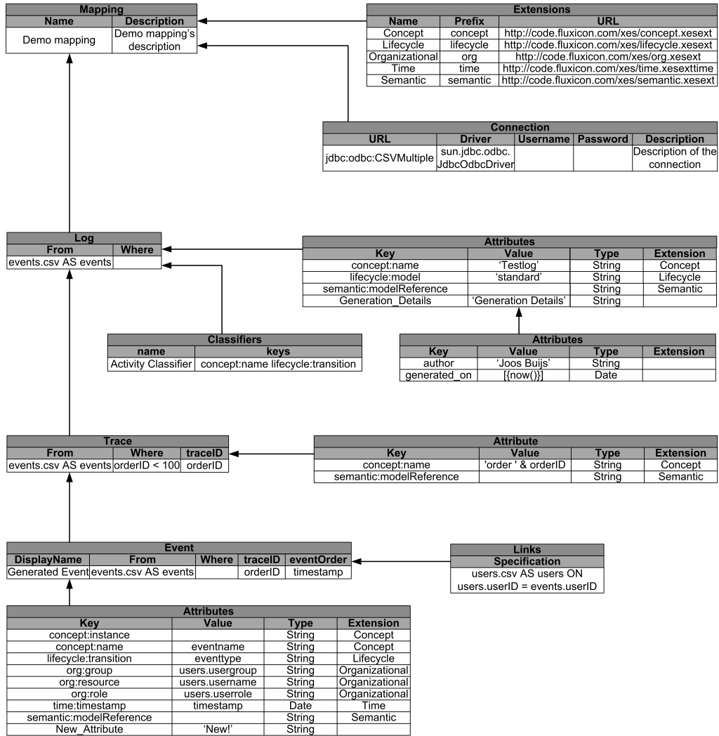
Figure 4.2: An instance of the class diagram for the example conversion definition.
