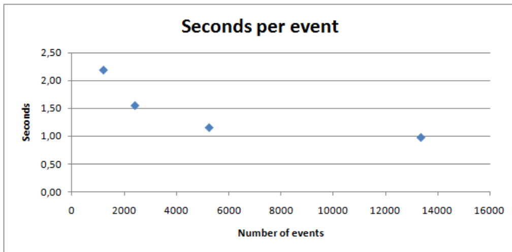
Figure 6.11: Case study 2: Time required per event.
