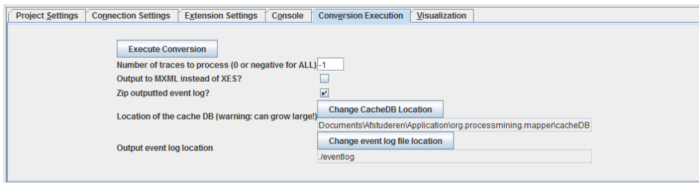
Figure 5.7: Execution settings tab.
