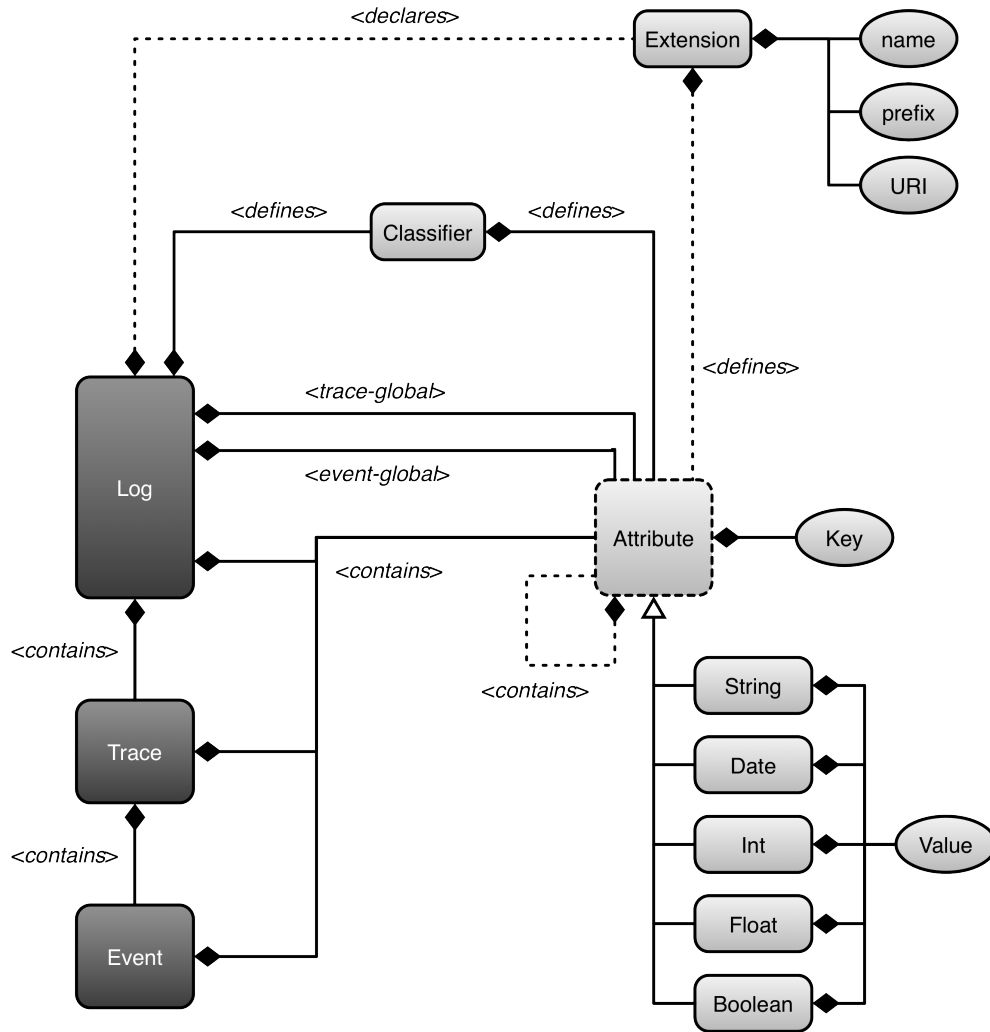
Figure 2.3: XES meta model
