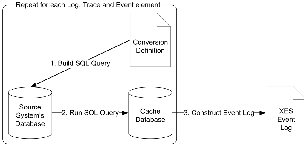
Figure 5.13: The three execution phases of the application.
