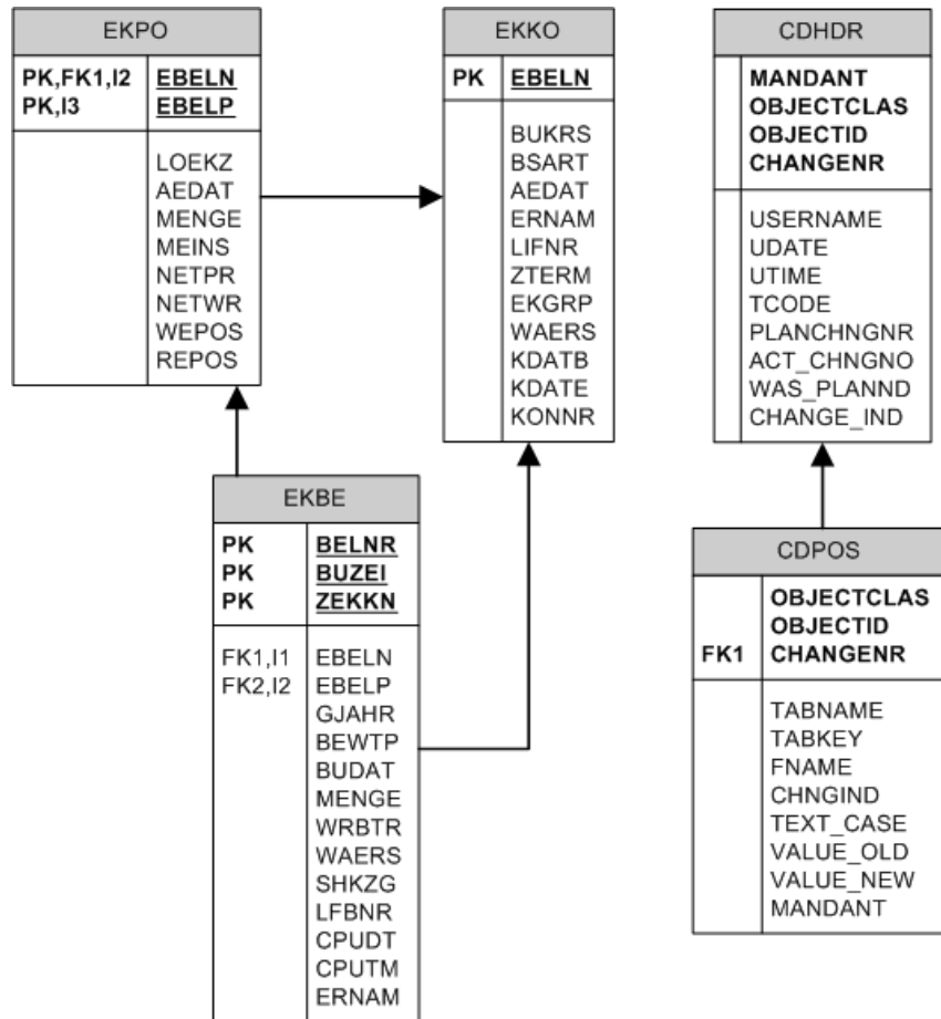
Figure 2.1: Procurement part of an SAP data model
