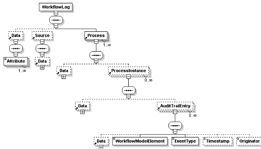
Figure B.1: MXML meta model
