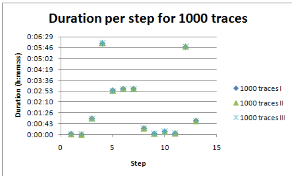
(b) Case study 1: Time per execution step for 1000 traces.
