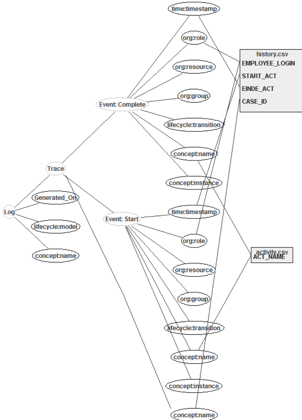
Figure 6.8: Conversion visualization for case study 2.
