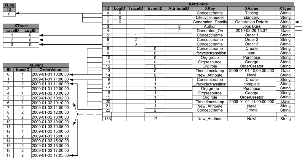
Figure 4.6: Intermediate database instance.
