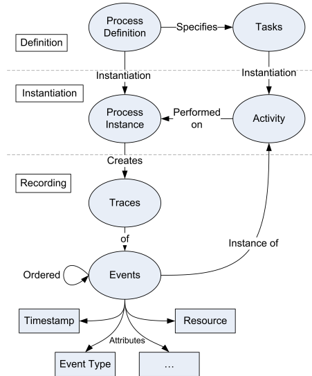
Figure 2.2: General event log structure.
