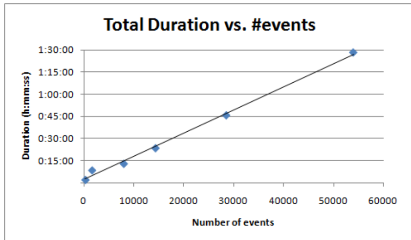
(b) Case study 1: Conversion duration versus number of events.
