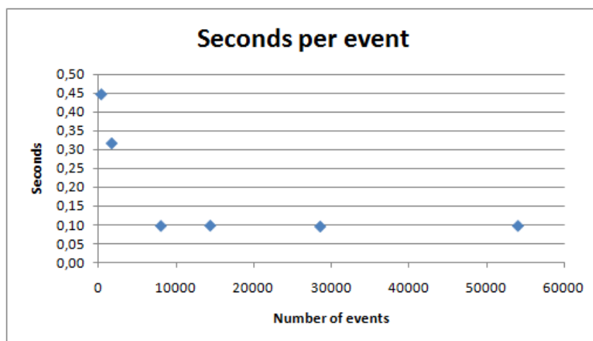
(c) Case study 1: Time required per event.
