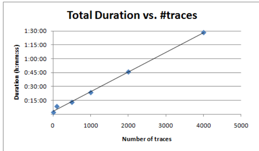
(a) Case study 1: Conversion duration versus number of traces.
