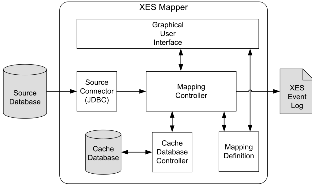
Figure 5.1: The environment of the application
