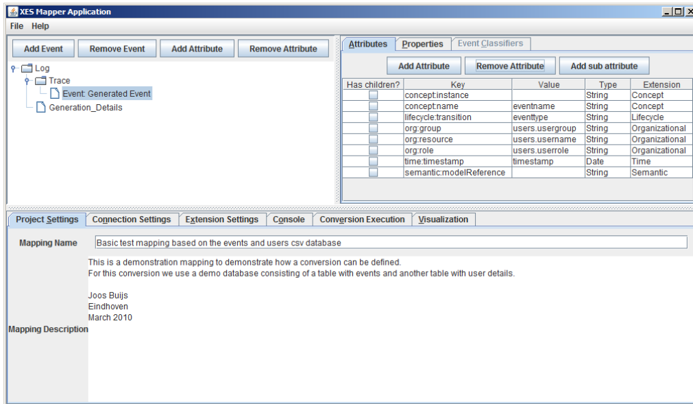
Figure 5.3: Graphical user interface of the application.
