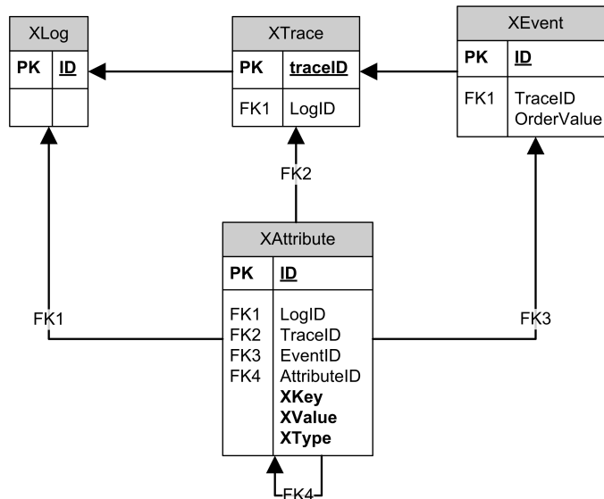
Figure 4.5: Intermediate database structure.
