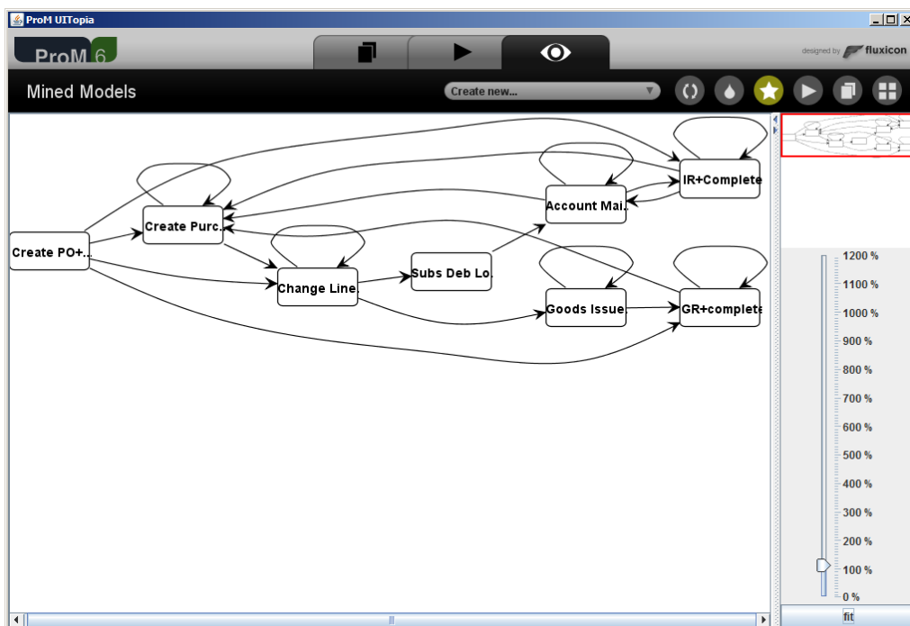
Figure 6.7: Case study 1 Heuristic miner model
