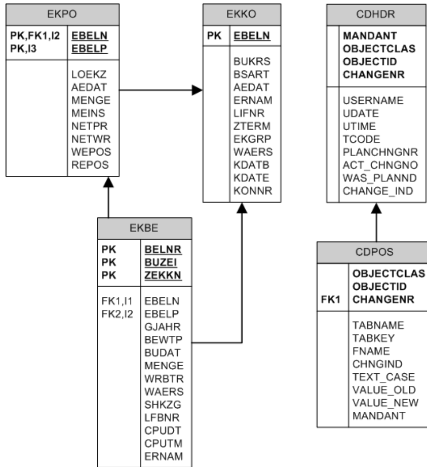
Figure 6.1: SAP source data structure
