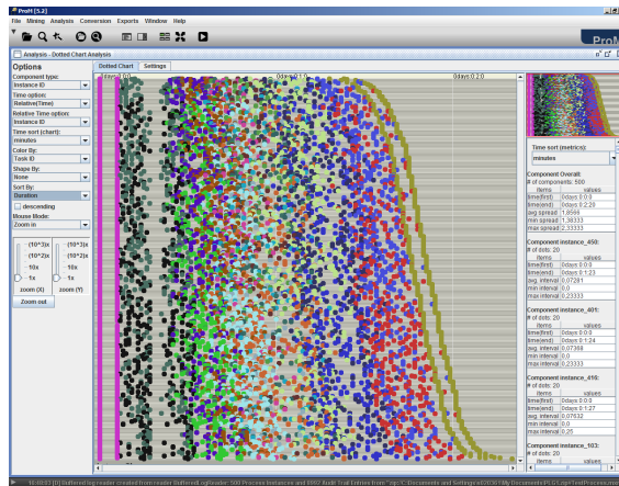
Figure 2.7: ProM 5.2 Dotted Chart result.
