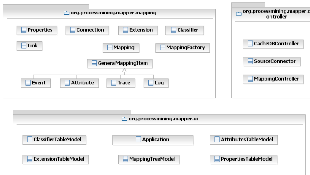
Figure 5.2: Class diagram of the application.
